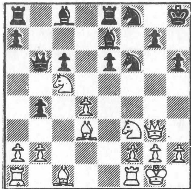
394 After 18...Kh8
